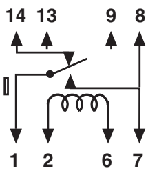
Figure M SPDT Without diode
