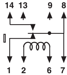
Figure P SPDT Without diode
